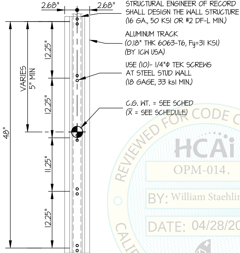
ELEVATION AT WALL PLATE (STEEL STUD WALL SHOWN)
