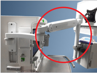
UL180-BV-W3-A1-DB2NK The Ultra 180 arm configured with a Drop Post to support the Nihon Kohden LifeScope G9 mobile monitor. The arm and device are mounted to a Mindray A7 Anesthesiology Workstation.
