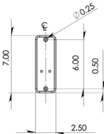
WALL PLATE
